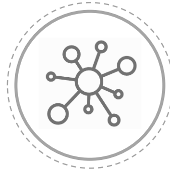
Analytics
